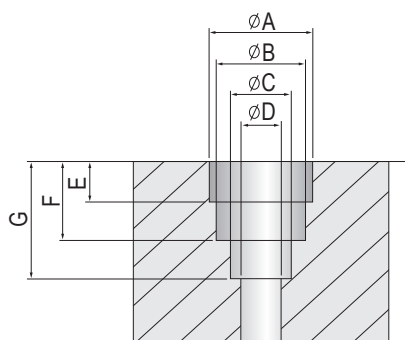
Cavity Dimension
